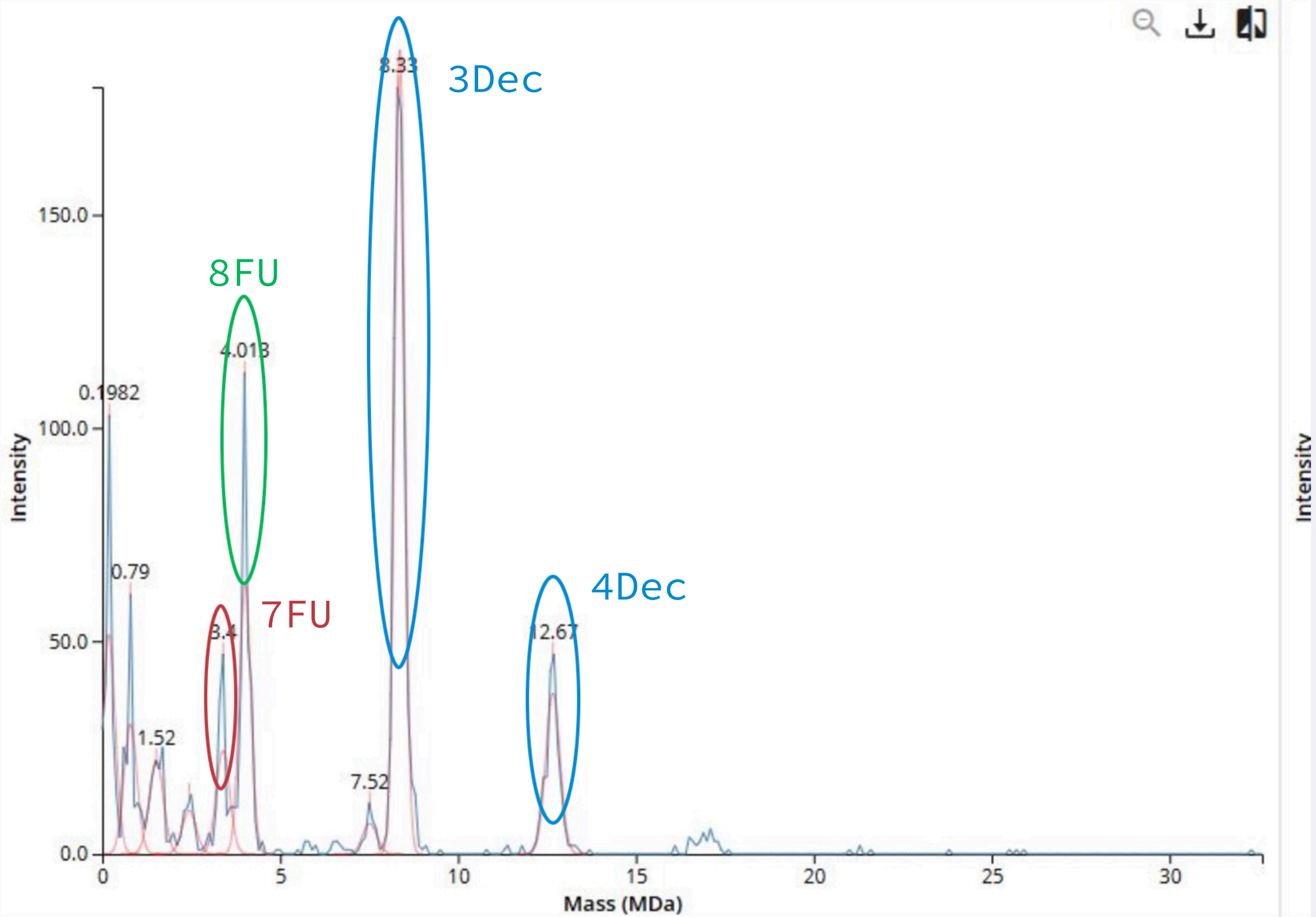
Figure 7. Mass spectrum of Keyhole Limpet Hemocyanin (KLH) acquired on the CDMS.
